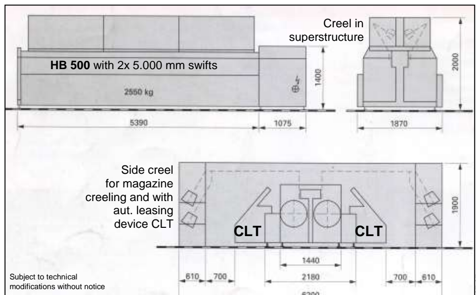
Dimensional drawing (measurements in mm)
